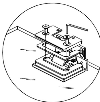
Figure 5 - Adjusting the screws
