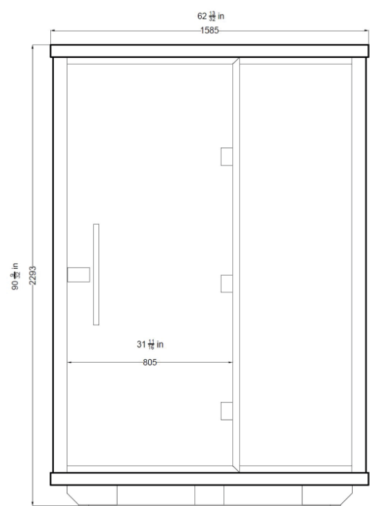
Figure 2 - Sauna front view
