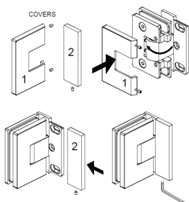
Figure 6 - Cover removal
