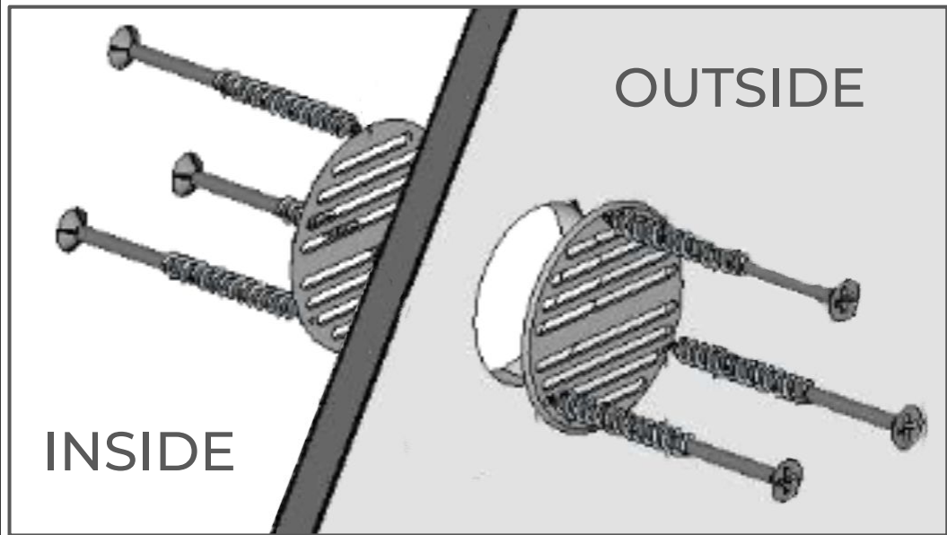
BOTTOM VENTILATION OPENING
